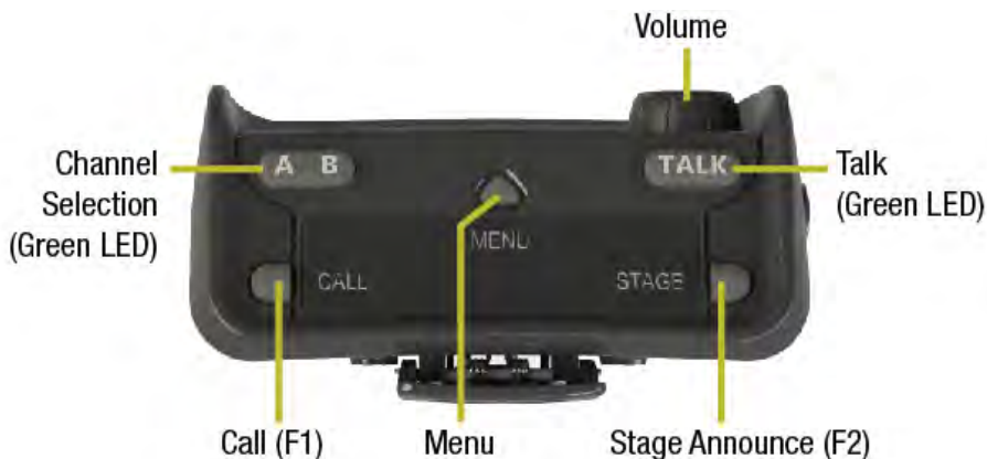
Figure 11 CRP-12 Top View
