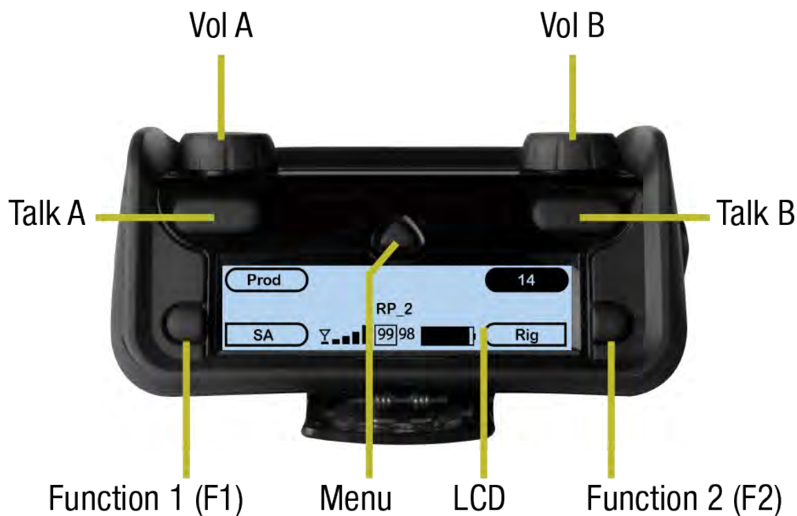
Figure 10 CRP-22 Top View
