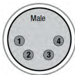
Figure 9 4-Pin Male XLR Pin Out
