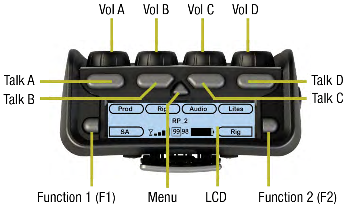
Figure 7 CRP-44 Top View
