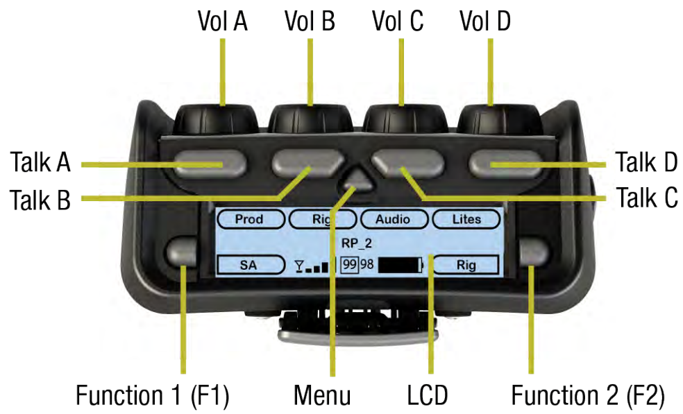
Figure 20 CRP-44 Top View
