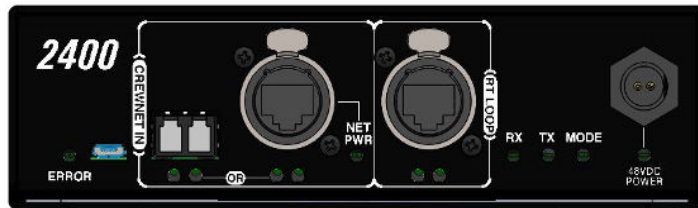
CRT-2400-IPR / CRT-2400CE-IPR* 2.4GHz Radio Transceiver (Bottom View)
